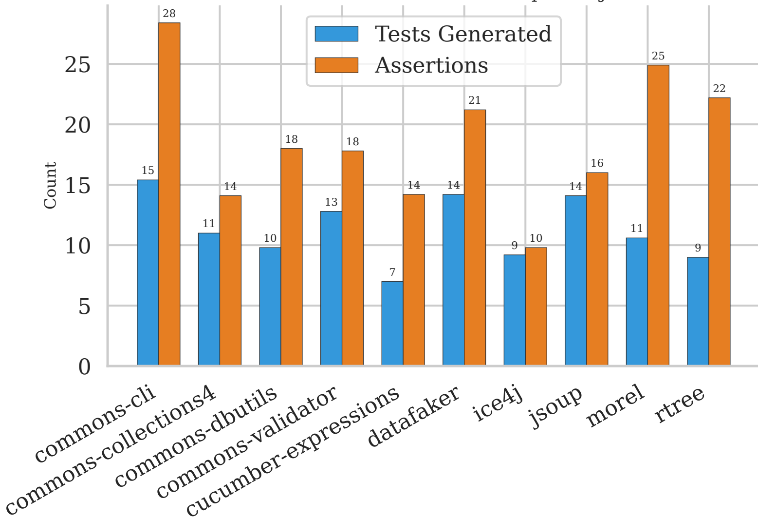
Tests and Assertions Generated per Project
