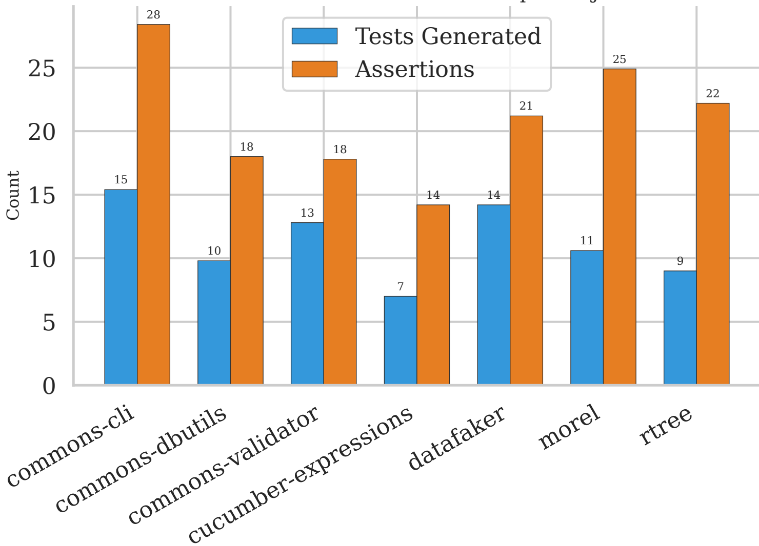
Tests and Assertions Generated per Project
