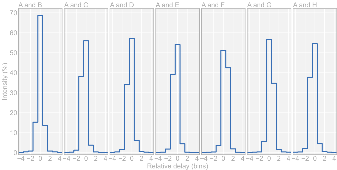
xHPTDC8 cable delay histograms
