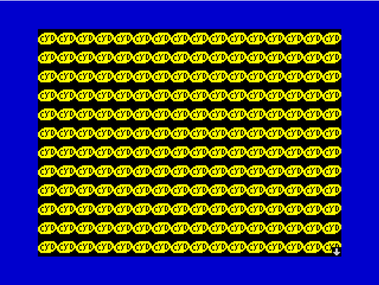
Figure 36: BLIT
