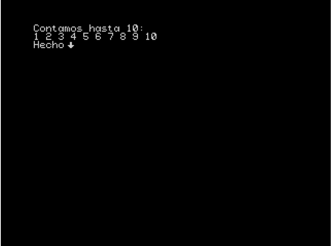
Figure 32: While
