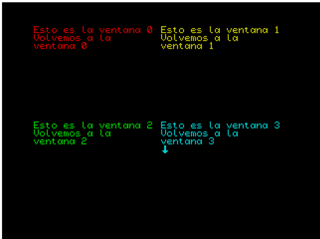
Figure 40: WINDOW
