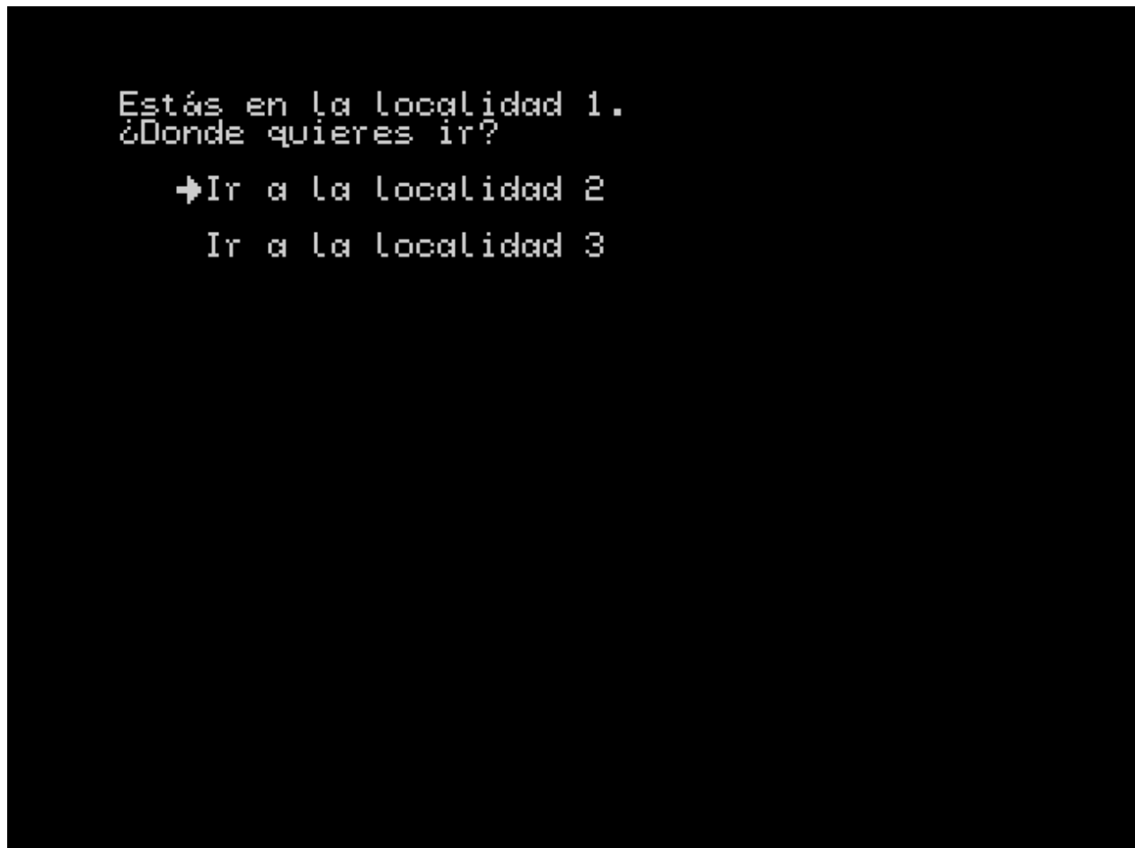
Figure 11: Tidy menu
