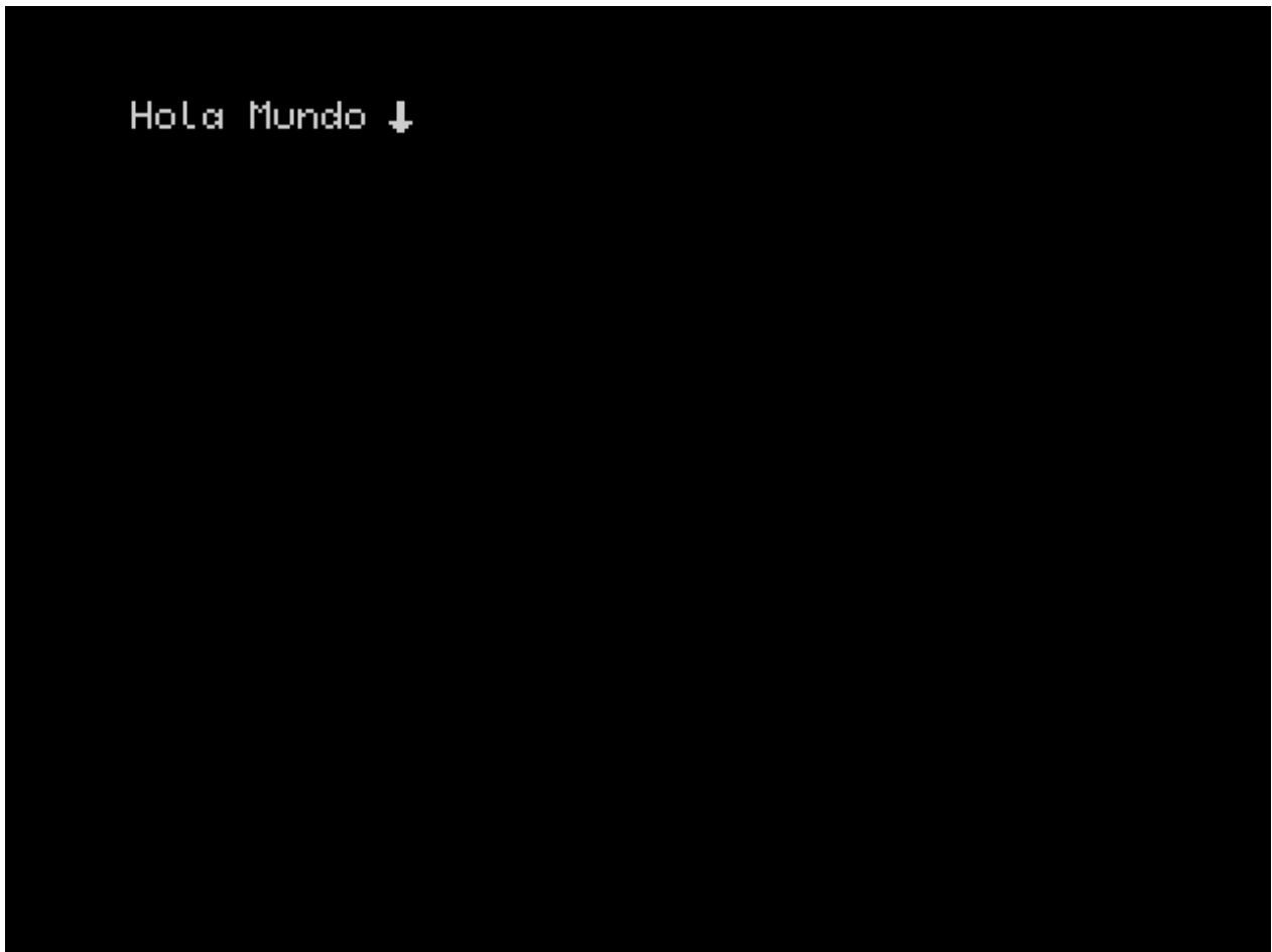
Figure 5: Screen 3
