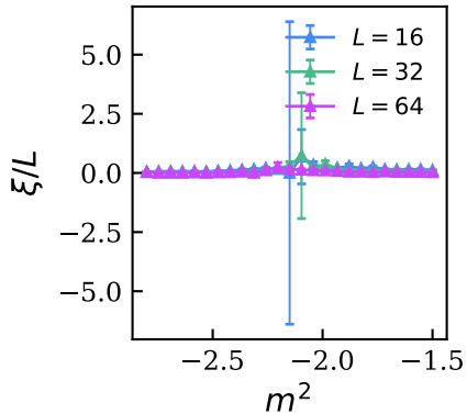
\xi/L Crossing
