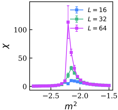
Susceptibility
