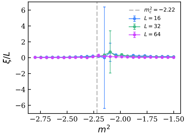
\xi/L Crossing
