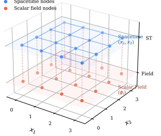
FIG. 1. 3D view of the heterogeneous bipartite graph for a 4 \times 4 lattice. Blue spheres (upper plane): spacetime nodes with coordinate features (x_1, x_2) . Orange spheres (lower plane): scalar field nodes with \phi values. Solid blue lines: adjacency edges encoding lattice connectivity. Dashed orange lines: inhabits edges coupling each field node to its spacetime site. Reverse inhabits edges (not shown) enable bidirectional message passing.
