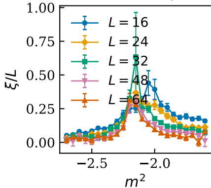
\xi/L Crossing
