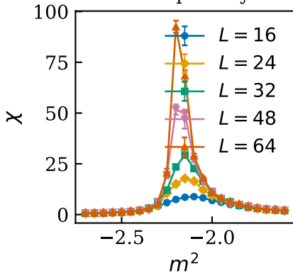
Susceptibility
