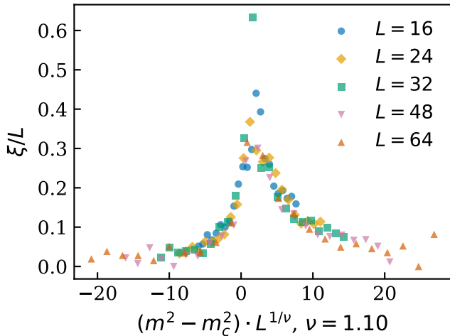
Scaling Collapse: \nu = 1.10
