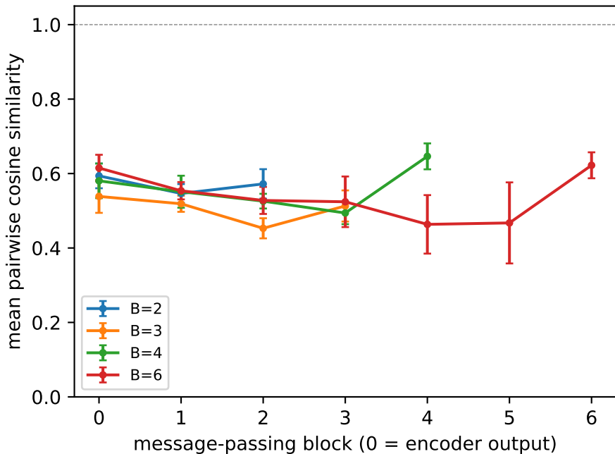
Variant C spacetime embeddings, L=16 , \beta=2
