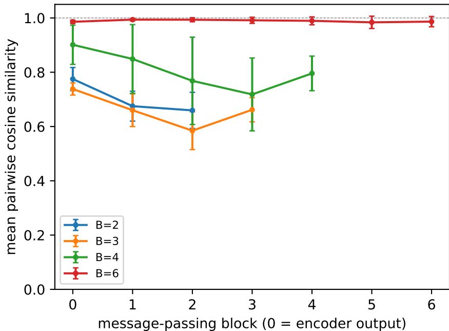
Variant C spacetime embeddings, L=16 , \beta=4
