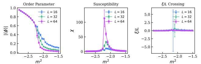
FIG. 3. Finite-size scaling results for \lambda = 0.5 . Left: Order parameter |\phi| showing progressive sharpening of the phase transition with increasing L . Center: Susceptibility \chi with peaks growing as \chi_{\text{max}} \sim L^{\gamma/\nu} and converging toward m_c^2 . Right: Correlation length ratio \xi/L with crossing of the L = 16 and L = 32 curves at m_c^2 = -2.22 \pm 0.24 . Error bars are binned jackknife errors with bin sizes set by the measured \tau_{\text{int}} .
