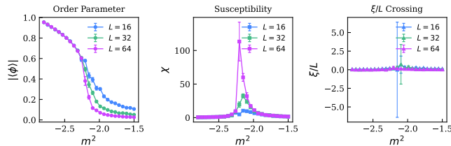
FIG. 2. Finite-size scaling results for \lambda = 0.5 . Left: Order parameter |\phi| showing progressive sharpening of the phase transition with increasing L . Center: Susceptibility \chi with peaks growing as \chi_{\max} \sim L^{\gamma/\nu} and converging toward m_c^2 . Right: Correlation length ratio \xi/L with crossing of the L = 16 and L = 32 curves at m_c^2 = -2.22 \pm 0.24 . Error bars are binned jackknife errors with bin sizes set by the measured \tau_{\text{int}} .
