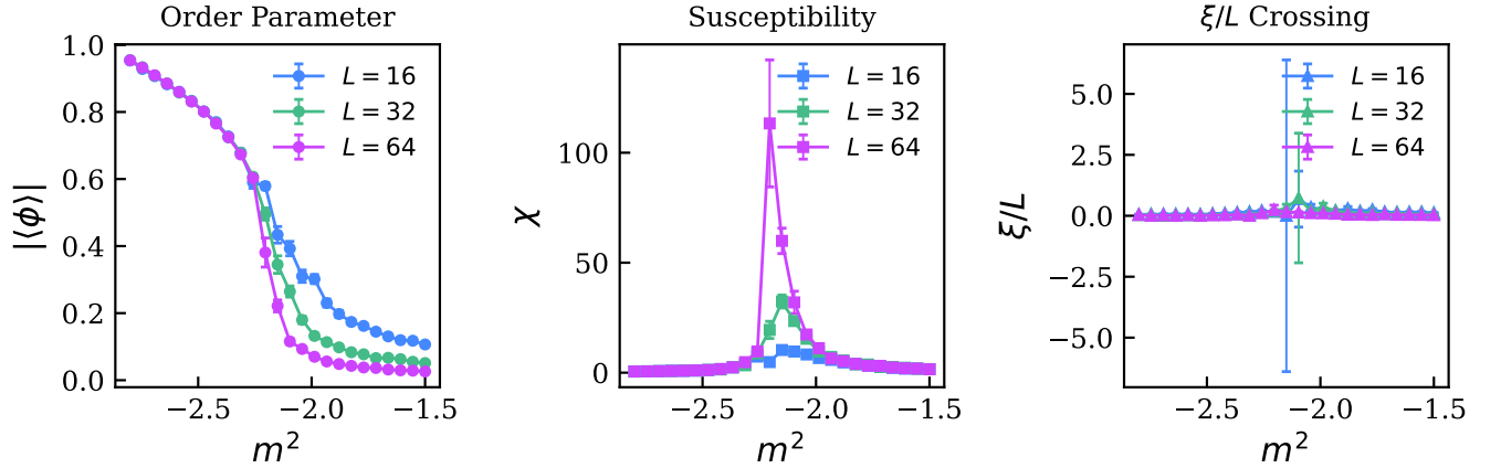
FIG. 3. Finite-size scaling results for \lambda = 0.5 . Left: Order parameter |M| showing progressive sharpening of the phase transition with increasing L . Center: Susceptibility \chi with peaks growing as \chi_{\max} \sim L^{\gamma/\nu} and converging toward m_c^2 . Right: Correlation length ratio \xi/L with crossing of the L = 16 and L = 32 curves at m_c^2 = -2.22 \pm 0.24 . Error bars are binned jackknife errors with bin sizes set by the measured \tau_{\text{int}} .
