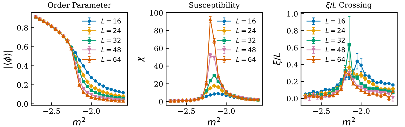
FIG. 3. Finite-size scaling of the cluster ensembles at \lambda = 0.5 . Left: order parameter |M| , sharpening with L . Center: susceptibility \chi , with peaks growing as \chi_{\max} \sim L^{\gamma/\nu} . Right: correlation-length ratio \xi/L , whose curves cross near m_c^2 = -2.217(3) . Error bars are binned jackknife errors with bin sizes set by the measured \tau_{\text{int}} ; per- L markers are colorblind-distinct.
