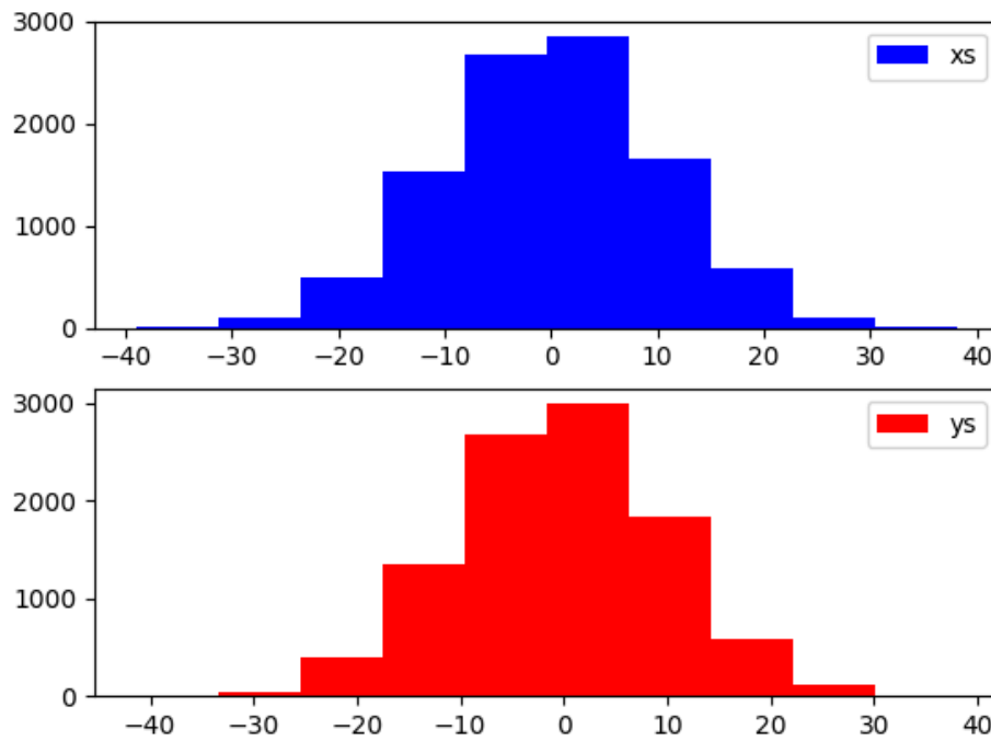
Histogram 2 D
