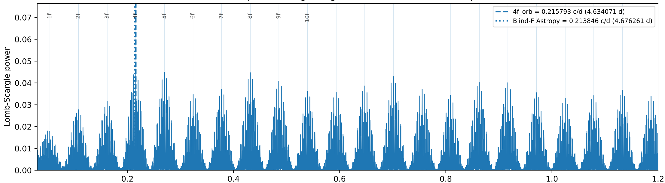
B. Before eclipse masking: integer harmonics dominate the spectrum
