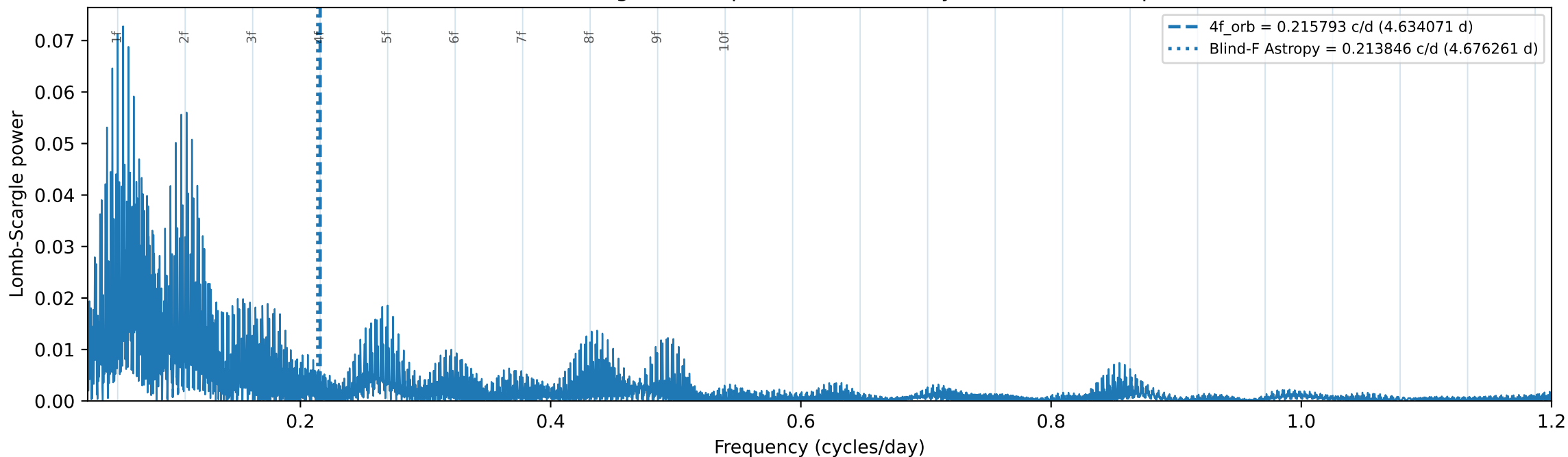
C. After masking both eclipses: the \sim 4.67 -day / 4f feature collapses
