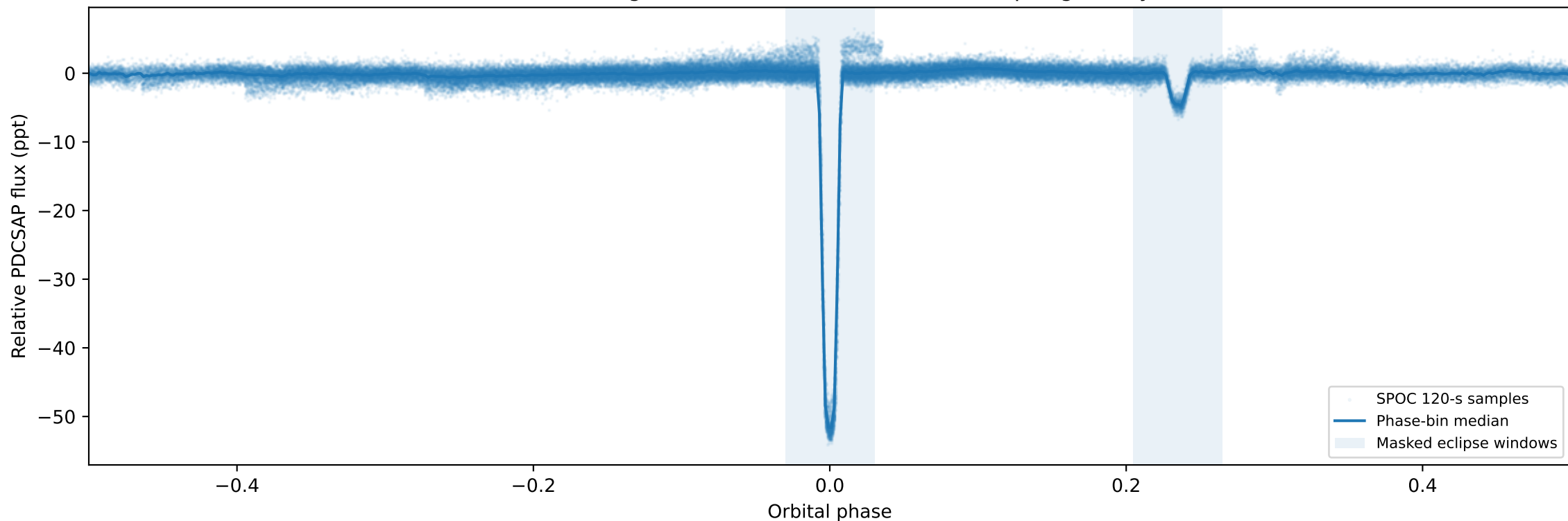
A. Multi-sector light curve folded on the known eclipsing-binary orbit
