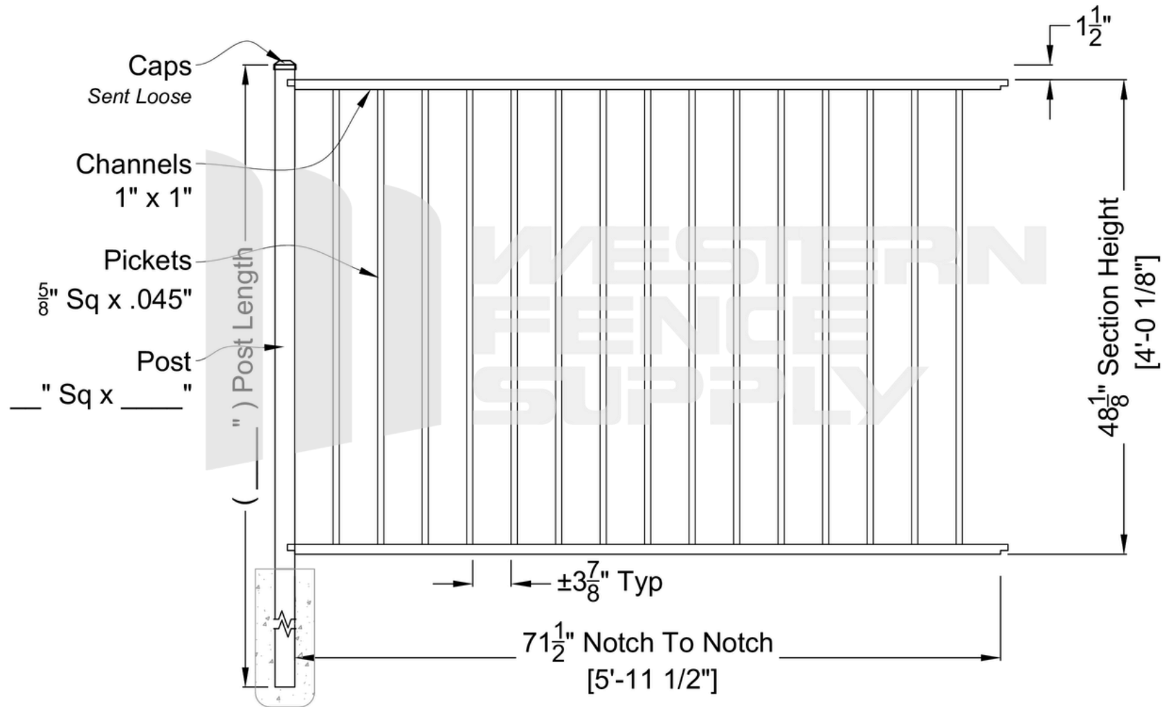
Aluminum Residential 2-Rail Smooth Bottom 4' x 6' Wide Panels
