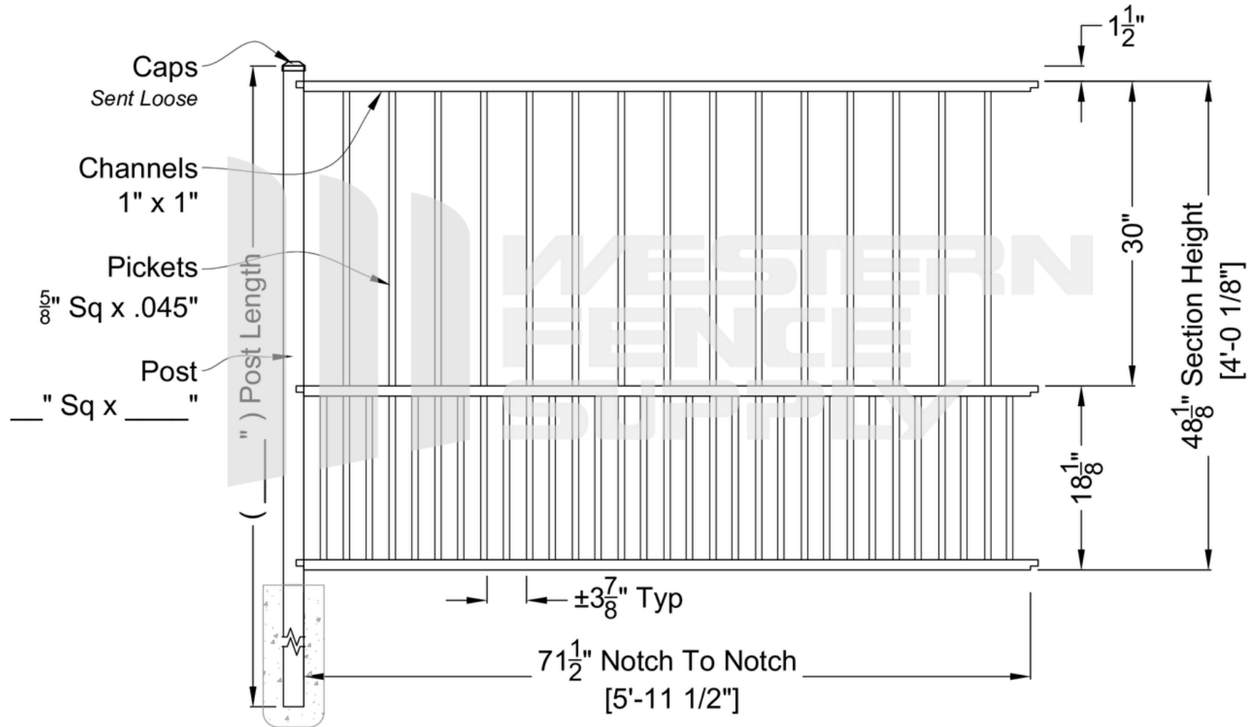
Aluminum Residential 3-Rail Puppy Picket 4' x 6' Wide Panels
