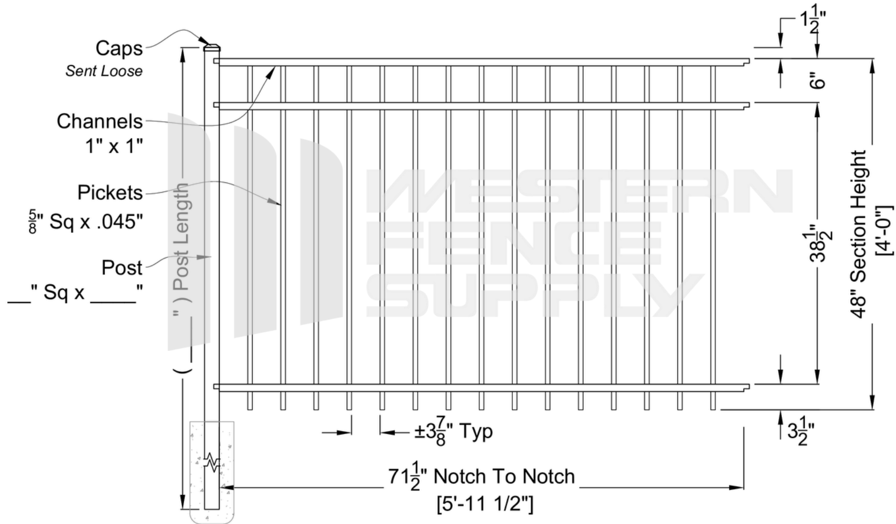
Aluminum Residential 3-Rail Rake Bottom 4' x 6' Wide Panels
