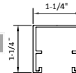
1-1/4" U Channel
