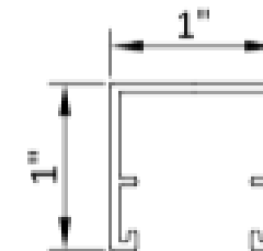
1" U Channel
