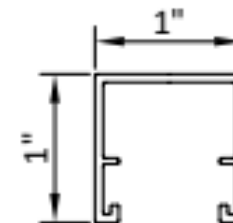
1" U Channel
