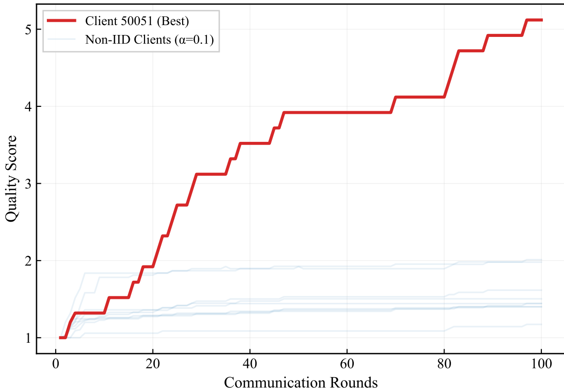
MEDMNIST Exp-A: Quality Score Dynamics
