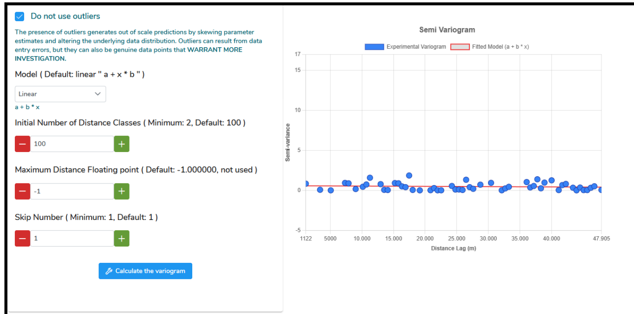
Figure 47 Publishing - Validation - Kriging Interpolation - Semi variogram
