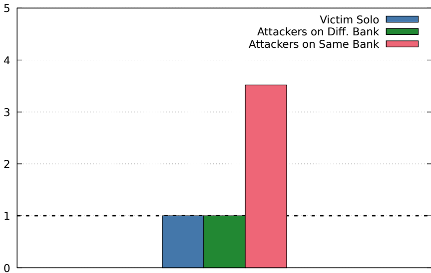
Normalized Victim Slowdown
