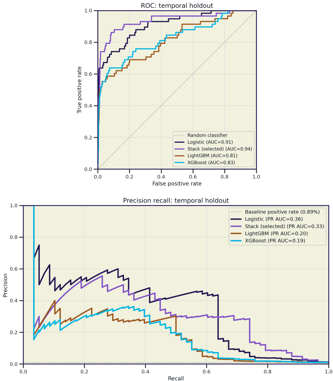
Figure 3: Discrimination on the temporal holdout. Top: ROC curves; the stack reaches AUC 0.94 and logistic regression 0.91, with tree-only baselines trailing. Bottom: precision–recall curves; logistic regression leads under prevalence-aware ranking with PR-AUC 0.36, the stack 0.33.
