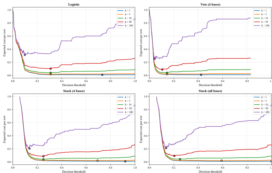
Figure 5: Business-utility curves: expected cost per row vs decision threshold across asymmetric cost ratios k = c_{\text{miss}}/c_{\text{false alarm}} . The recommended operating point (filled dot) is robust for k \in [3, 30] .
