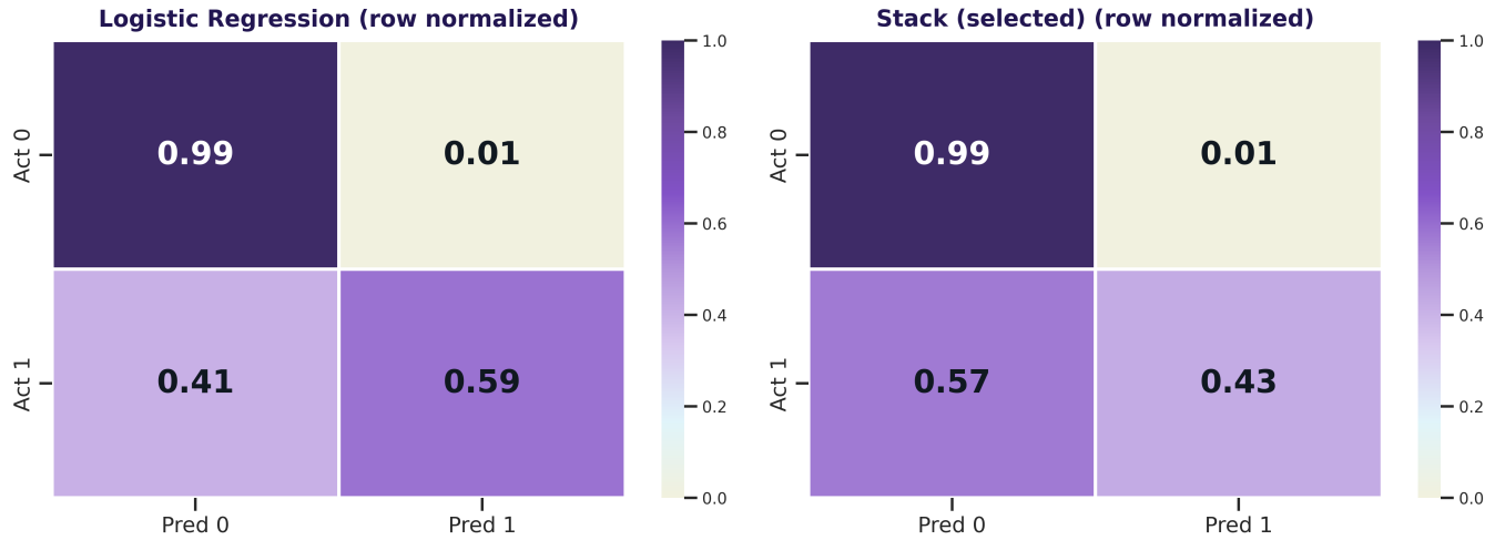
Confusion matrices: temporal holdout
