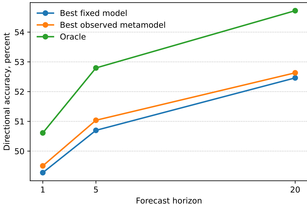
Fixed model, metamodel selection, and oracle directional accuracy
