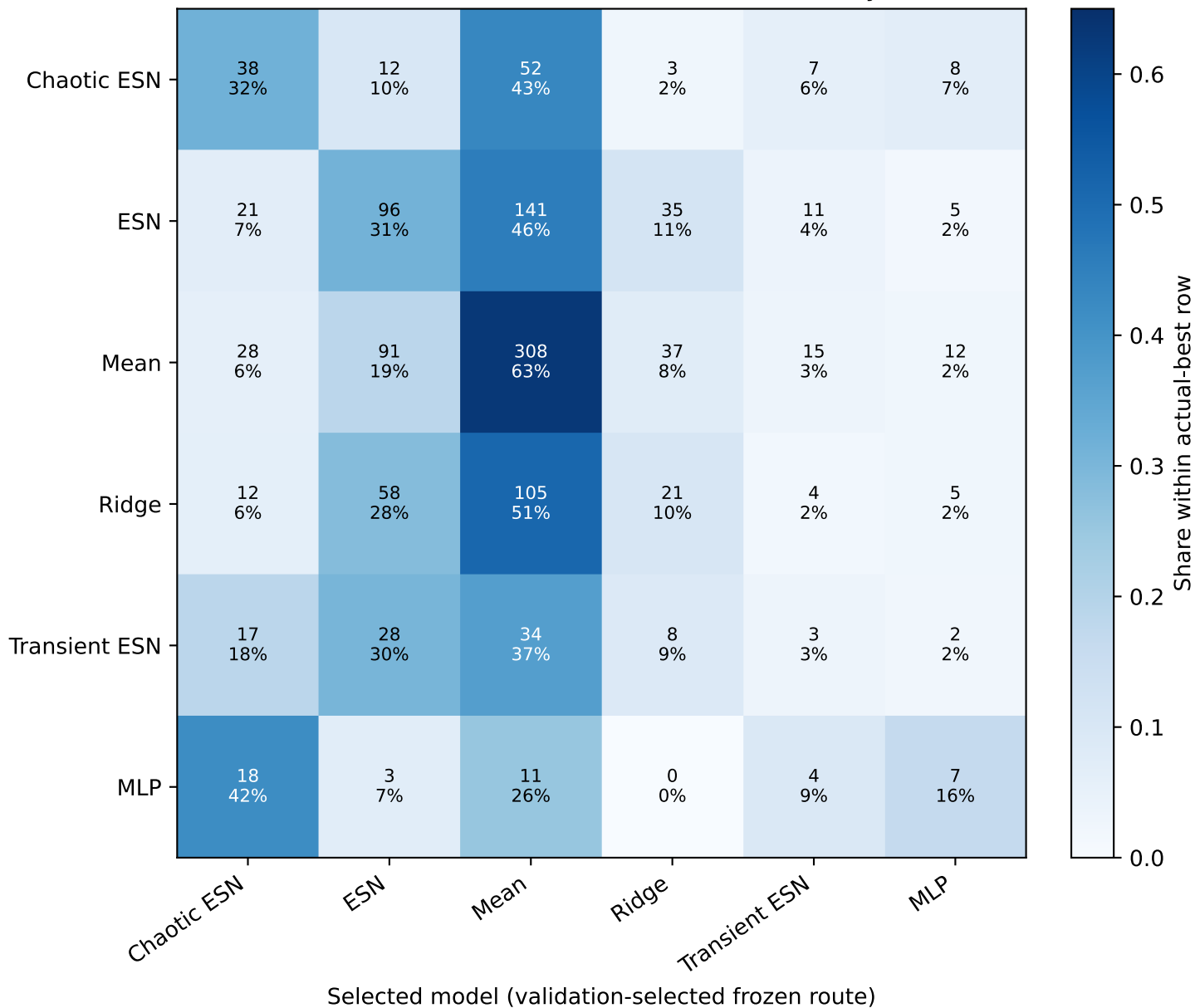
Pooled confusion matrix for h=5 directional accuracy (N=1,260)
