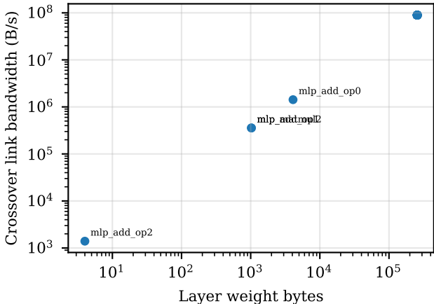
Per-layer pool/NMC crossover (cost model)
