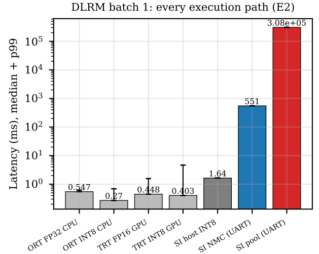
Fig. 4. E2 latencies (log scale; bar = median, whisker to p99).
