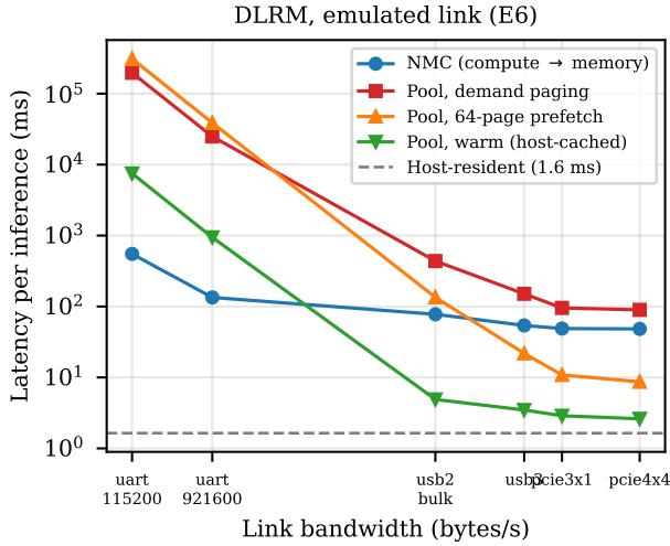
Fig. 5. E6 ( E ): latency per inference versus link bandwidth for NMC and three pool configurations. The crossover between NMC and prefetching pool lies between USB 2.0 and USB 3.
