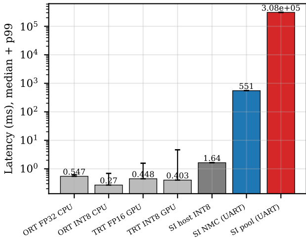
DLRM batch 1: every execution path (E2)
