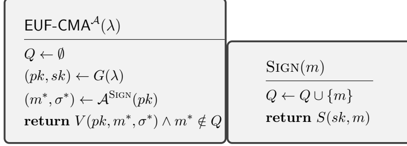
Figure 1: The EUF-CMA attack game for a signature scheme (G, S, V) . The adversary \mathcal{A} has oracle access to \text{SIGN} , which signs any requested message and records it in Q ; \mathcal{A} wins by outputting a valid signature on a message it never sent to \text{SIGN} .
