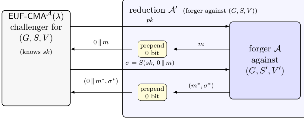
Figure 2: The security reduction drawn in the standard “box-within-a-box” style.
