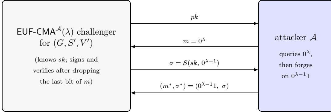
Figure 3: The forgery attack of the previous example. Unlike Figure 2, this is not a reduction: the attacker \mathcal{A} is a single program playing the EUF-CMA game directly against the modified scheme (G, S', V') , whose signing oracle and verifier both drop the last bit of a message.
