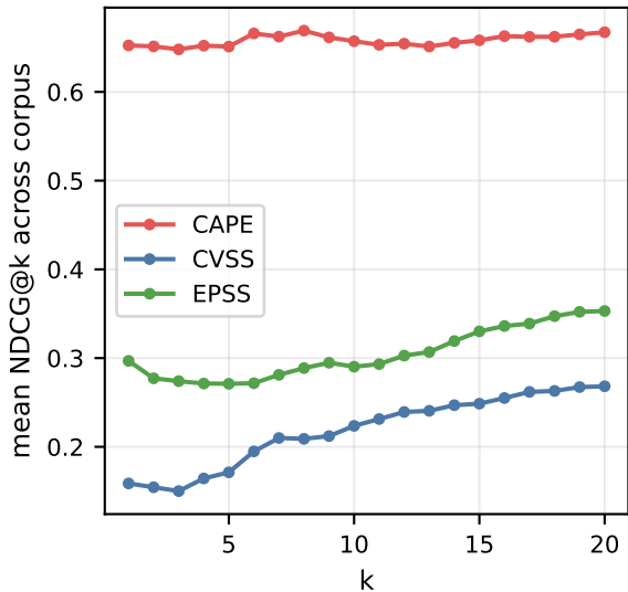
Ranking quality vs. cutoff k
