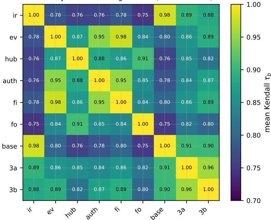
Centrality-variant rank agreement (30-case mean)
