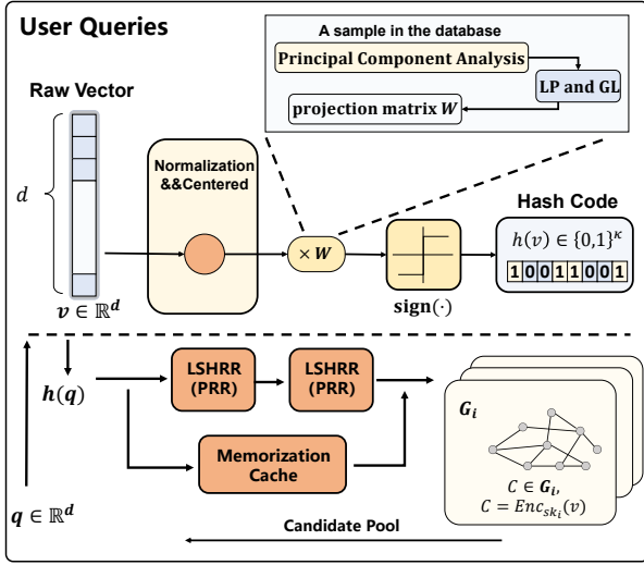
Fig. 3: Systematic illustration of the query flow.
