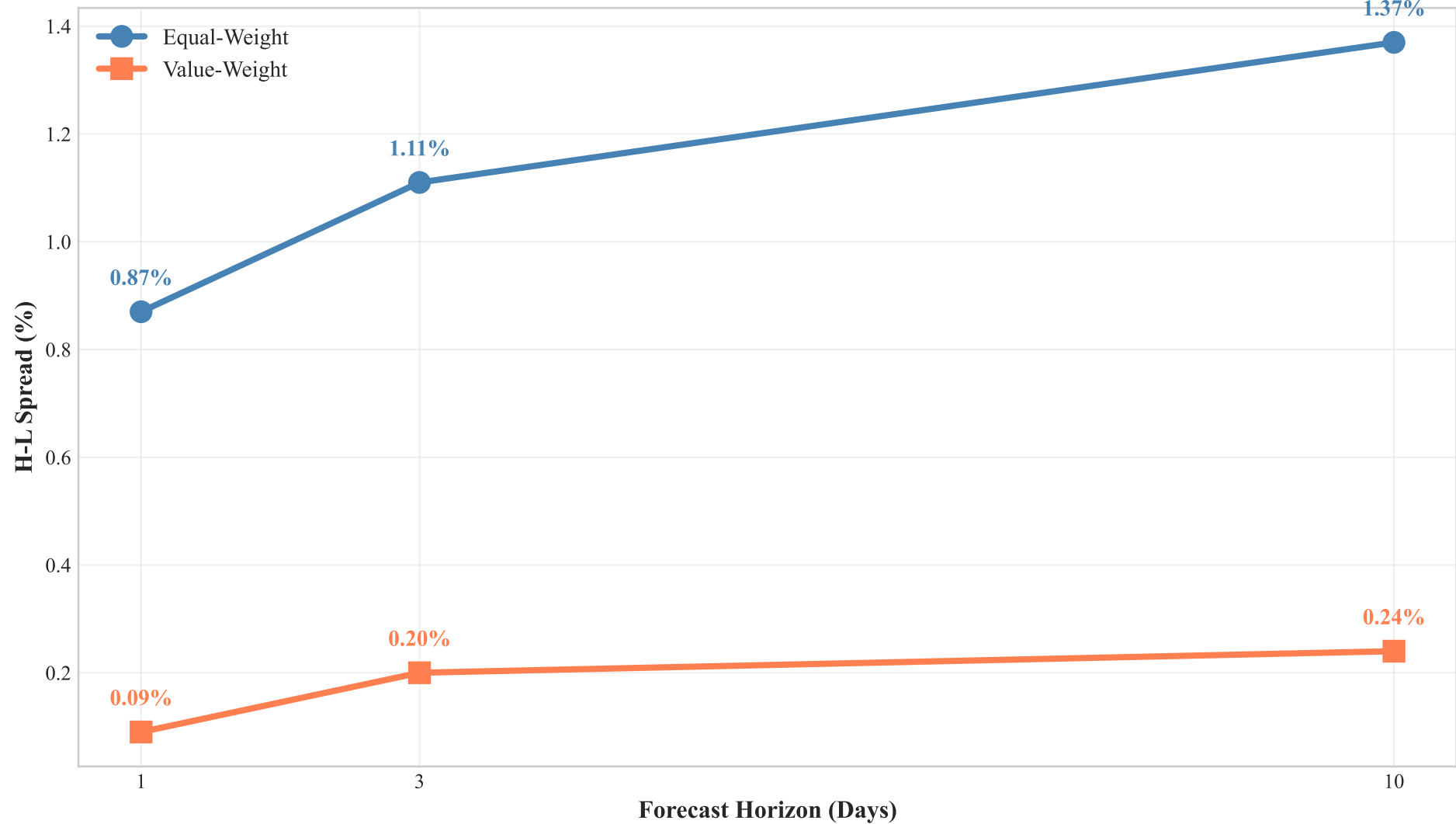
CNN Predictive Power Increases with Forecast Horizon
