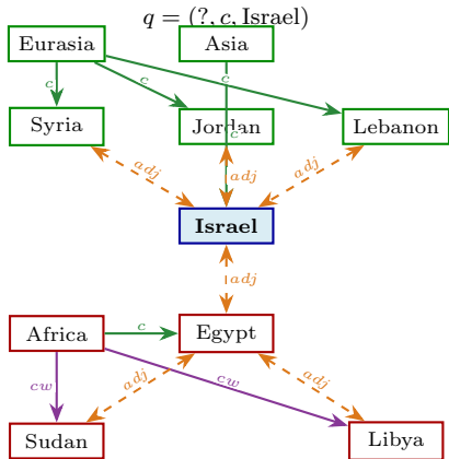
(a) Local KG
