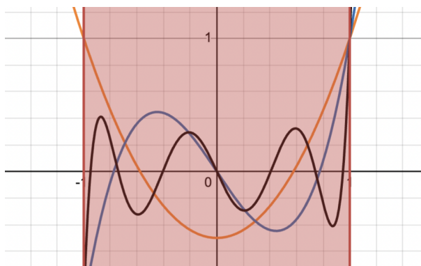
Figure 7.1: Legendre polynomials integrate to 0
