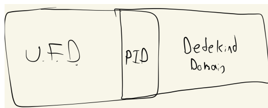
Figure 22.1: Venn diagram
