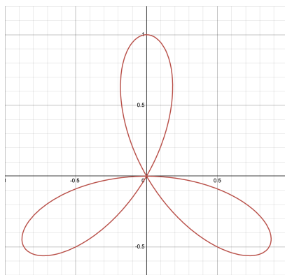
Figure 38.1: Three-Leaf Curve
