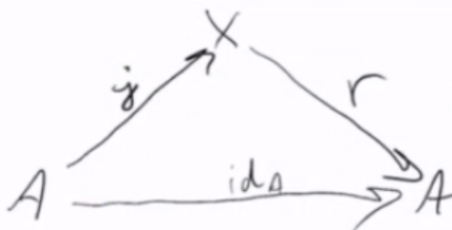
Figure 6.11: The retraction r gives a left inverse to the map induced by inclusion.
