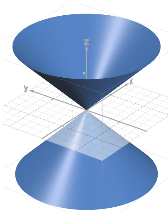
Figure 27.3: zero set of x^2 + y^2 - z^2
