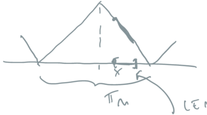
Figure 5.6: Demonstration of monotonicity
