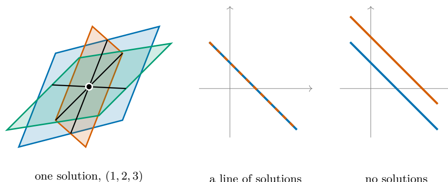
Figure 1: Three planes meeting in three lines that share one point, two equations describing the same line, and two parallel lines
