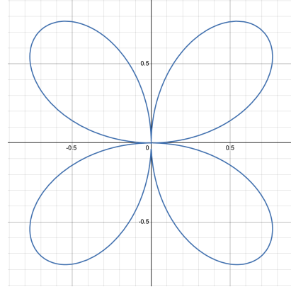
Figure 21.10: Four-Leaf Curve
