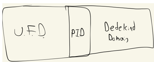
Figure 48.1: Venn diagram
