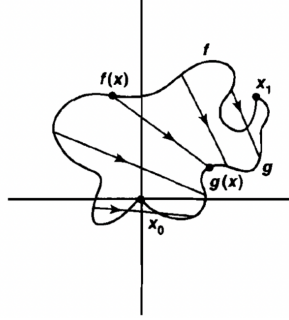
Figure 2.2: Convex space
