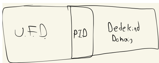
Figure 22.1: Venn diagram
