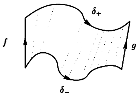
Figure 33.1: homotopy
