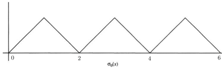
Figure 3.4: \sigma_0
