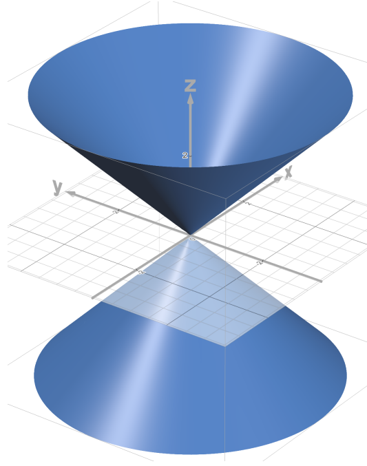
Figure 7.2: zero set of x^2 + y^2 - z^2
