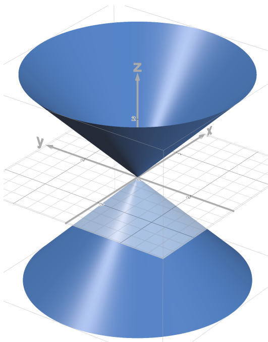
Figure 1.3: zero set of x^2 + y^2 - z^2
